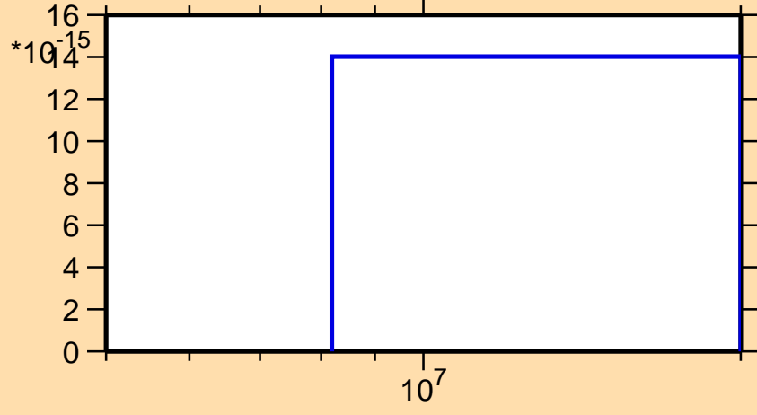
\sigma vs. E for ^{126}\text{I}(\text{mt117})
