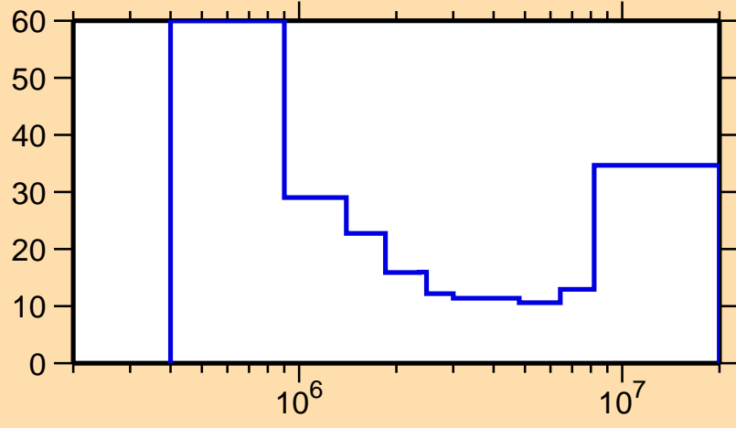
\Delta\sigma/\sigma vs. E for ^{126}\text{I}(n,n\text{cont.})
