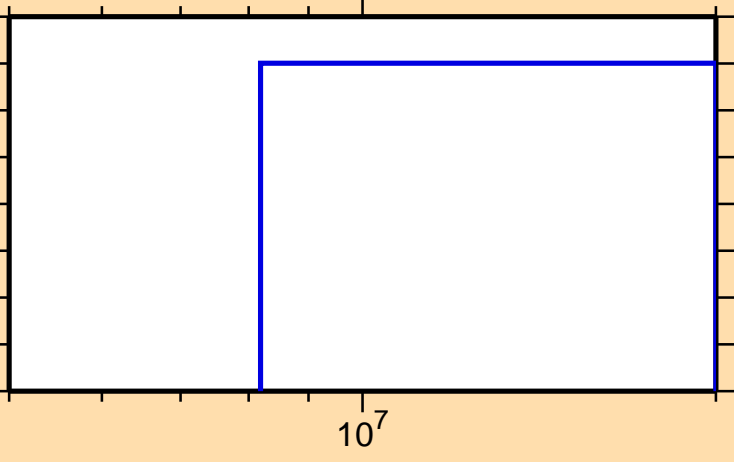
\sigma vs. E for ^{126}\text{I}(n,\text{He3})
