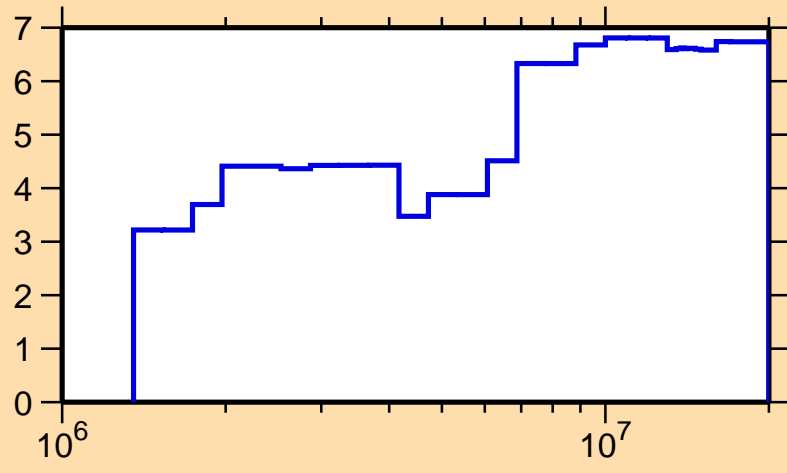
\Delta\sigma/\sigma vs. E for ^{127}\text{I}(n, el.)
