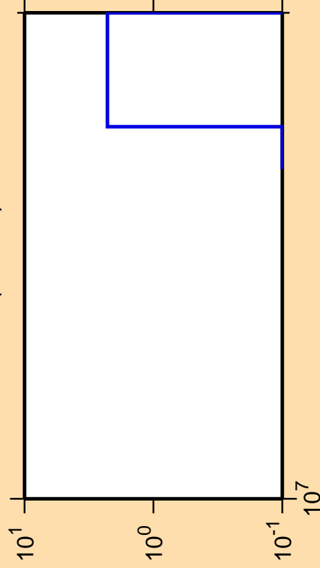
\Delta\sigma/\sigma vs. E for ^{127}\text{I}(\text{mt117})
