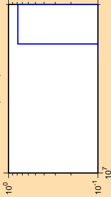
\Delta\sigma/\sigma vs. E for ^{127}\text{I} (mt 45)
