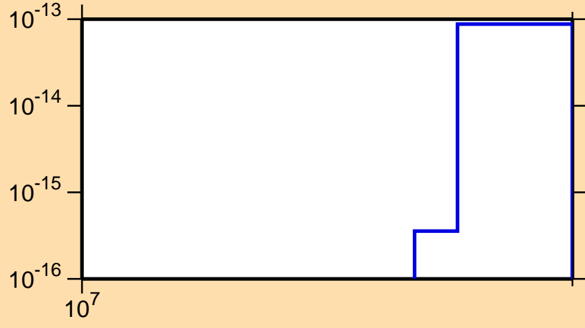
\sigma vs. E for ^{127}\text{I} (mt 45)
