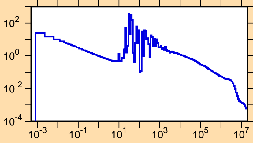
\sigma vs. E for ^{127}\text{I}(n,\gamma)
