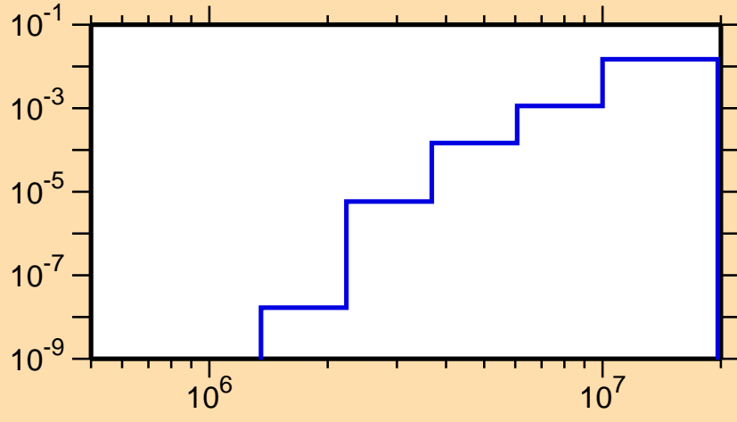
\sigma vs. E for ^{127}\text{I}(n,p)
