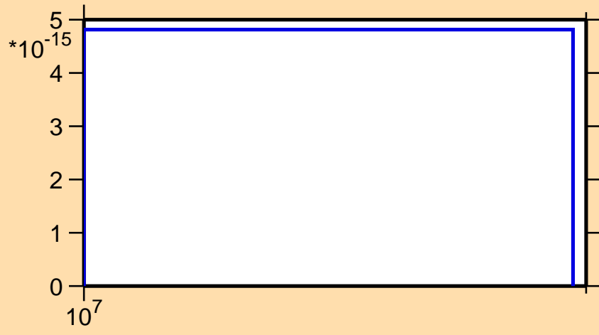
\sigma vs. E for ^{127}\text{I}(\text{mt117})
