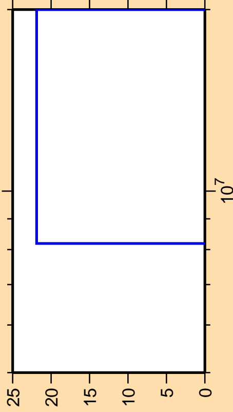
\Delta\sigma/\sigma vs. E for ^{127}\text{I}(n,n_1)
