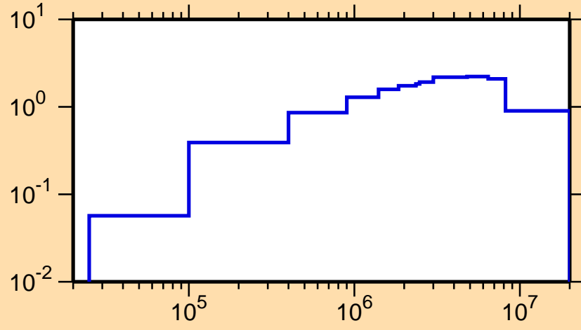
\sigma vs. E for ^{127}\text{I}(n,\text{inel.})
