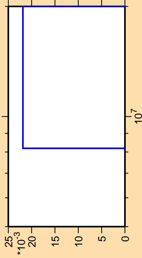
\Delta\sigma/\sigma vs. E for ^{127}\text{I}(\text{mt117})
