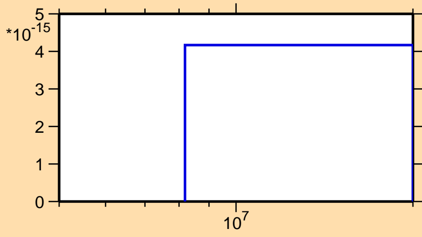
\sigma vs. E for ^{127}\text{I}(\text{mt117})
