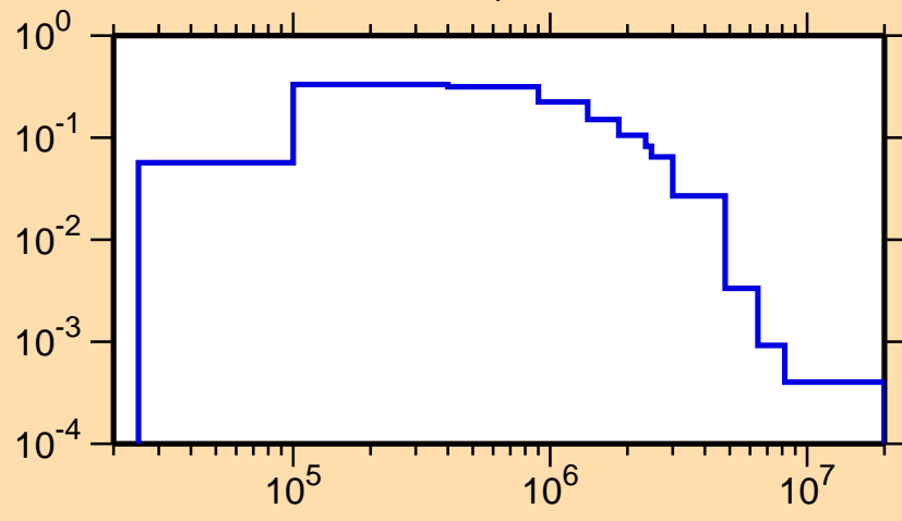
\sigma vs. E for ^{127}\text{I}(n,n_1)
