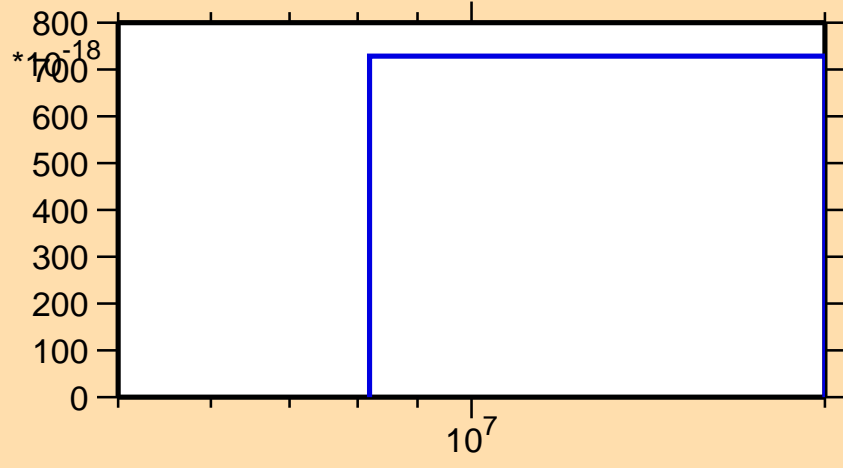
\sigma vs. E for ^{127}\text{I} (mt 45)
