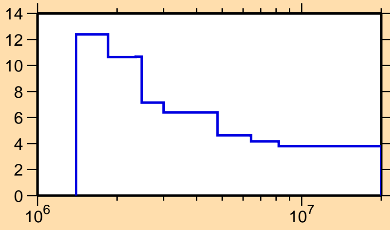
\Delta\sigma/\sigma vs. E for ^{127}\text{I}(n, nonel.)
