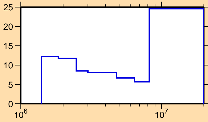
\Delta\sigma/\sigma vs. E for ^{127}\text{I}(n,n\text{cont.})
