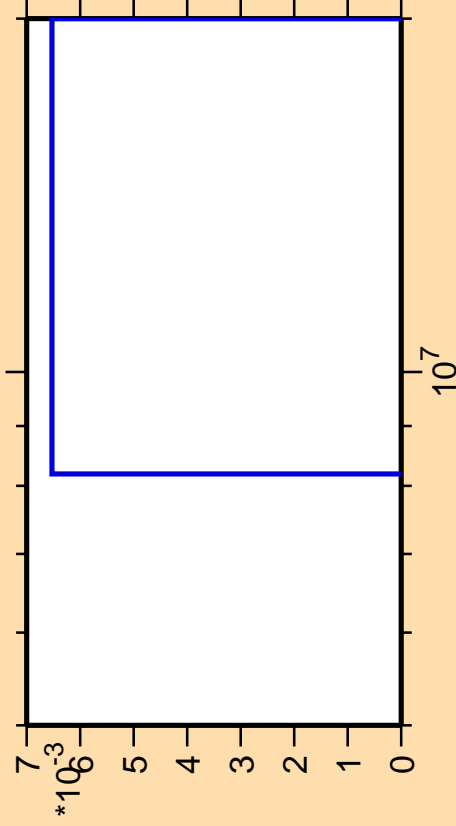
\Delta\sigma/\sigma vs. E for ^{127}\text{I} (mt 45)
