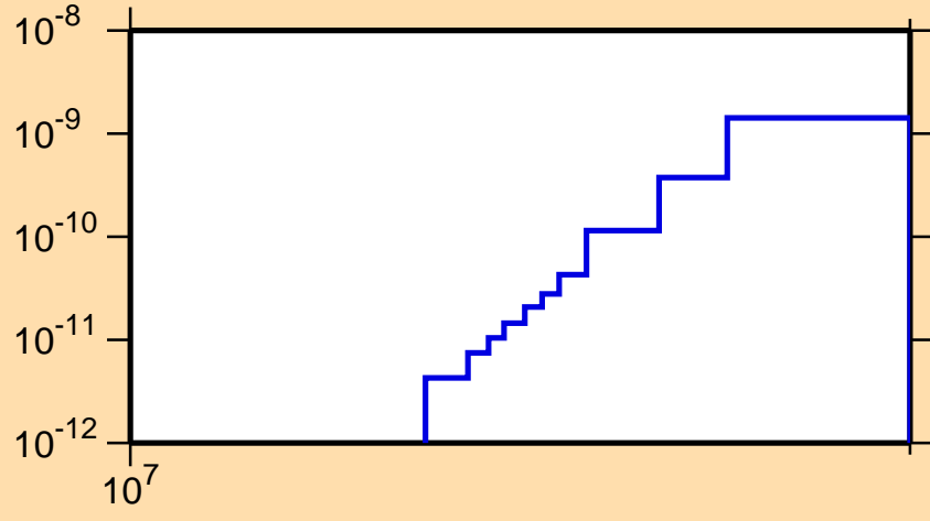
\sigma vs. E for ^{128}\text{I}(n,p\alpha)
