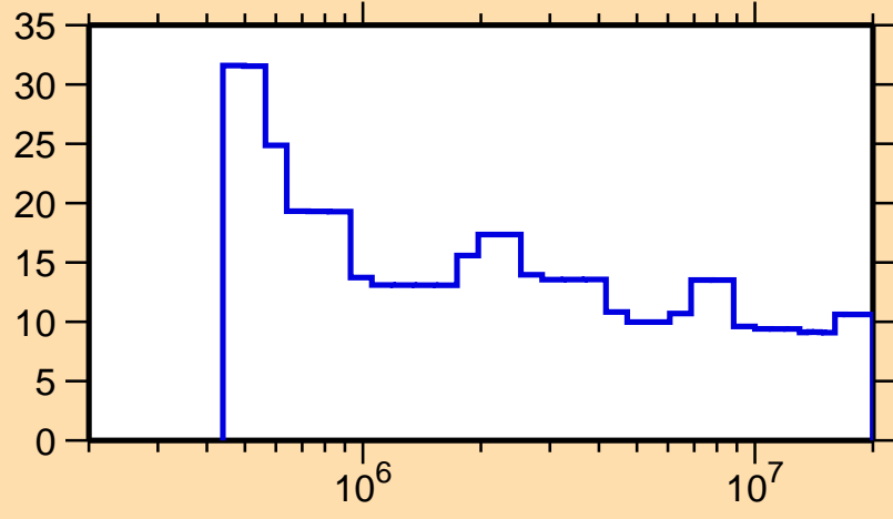
\Delta\sigma/\sigma vs. E for ^{128}\text{I}(n, el.)
