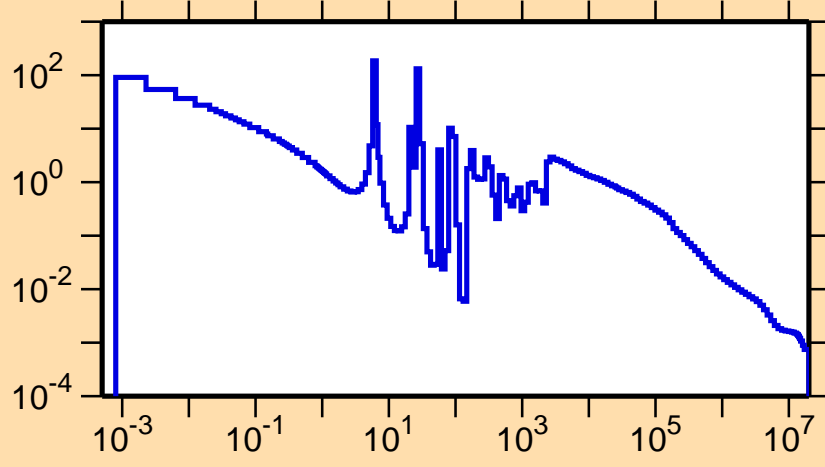
\sigma vs. E for ^{128}\text{I}(n,\gamma)
