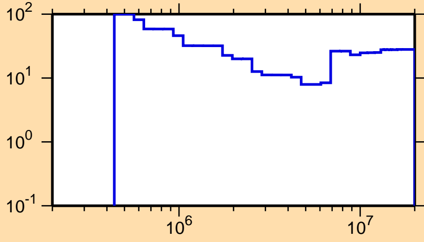
\Delta\sigma/\sigma vs. E for ^{128}\text{I}(n,n\text{cont.})
