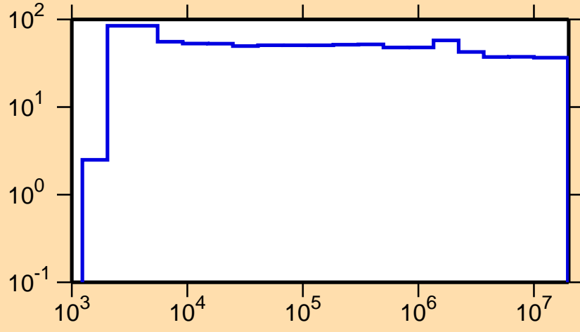
\Delta\sigma/\sigma vs. E for ^{128}\text{I}(n,p)
