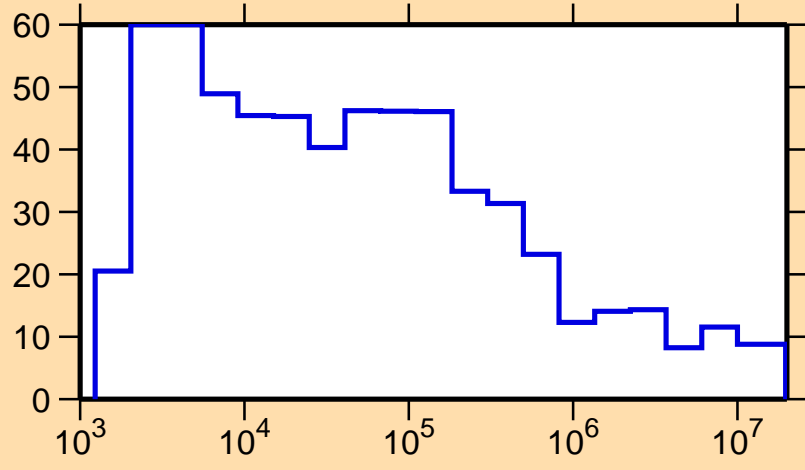
\Delta\sigma/\sigma vs. E for ^{128}\text{I}(n,el.)
