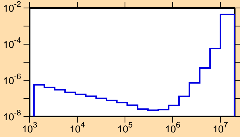
\sigma vs. E for ^{128}\text{I}(n,\alpha)
