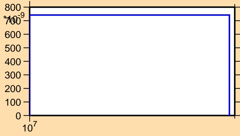
\sigma vs. E for ^{128}\text{I}(n,\text{nd})
