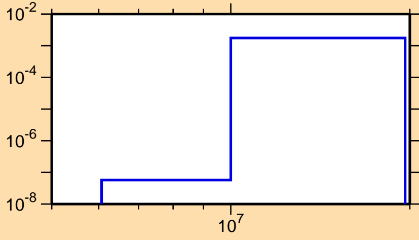
\sigma vs. E for ^{128}\text{I}(n,d)
