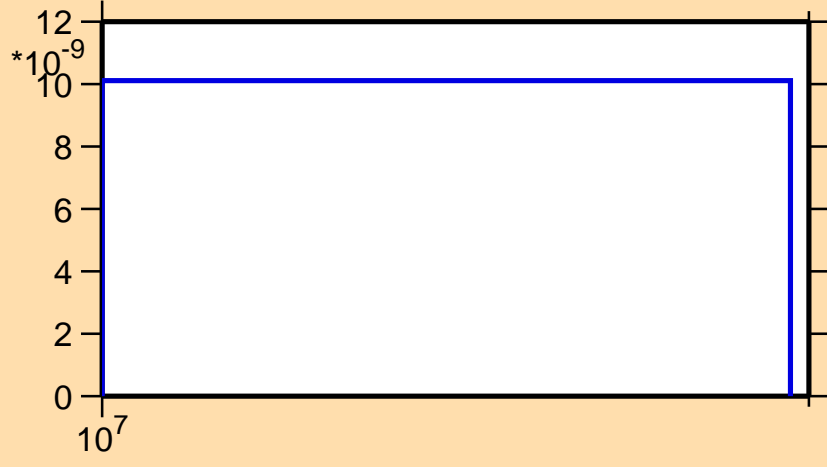
\sigma vs. E for ^{128}\text{I}(n,2n\alpha)
