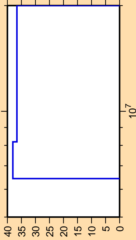
\Delta\sigma/\sigma vs. E for ^{128}\text{I}(n,p)
