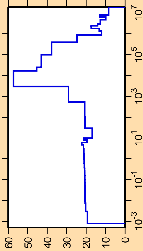
\Delta\sigma/\sigma vs. E for ^{128}\text{I}(n,\text{el.})
