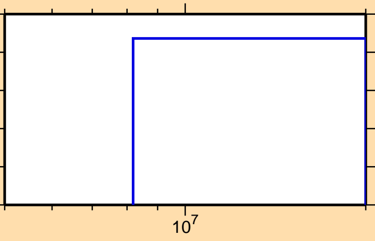
\sigma vs. E for ^{128}\text{I}(n,2np)
