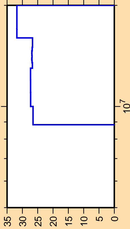
\Delta\sigma/\sigma vs. E for ^{129}\text{I}(n,n_1)
