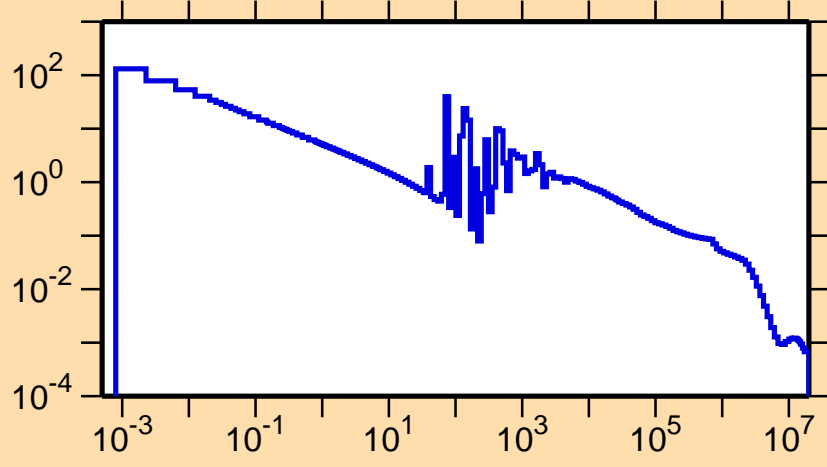
\sigma vs. E for ^{129}\text{I}(n,\gamma)
