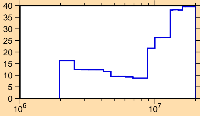
\Delta\sigma/\sigma vs. E for ^{129}\text{I}(n,n\text{cont.})
