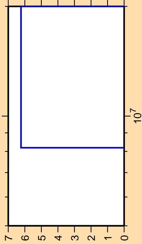
\Delta\sigma/\sigma vs. E for ^{129}\text{I}(n,2n)
