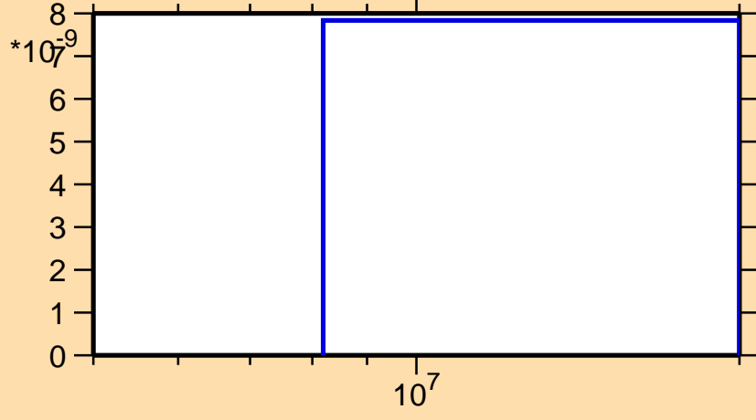
\sigma vs. E for ^{129}\text{I}(n,\text{nd})
