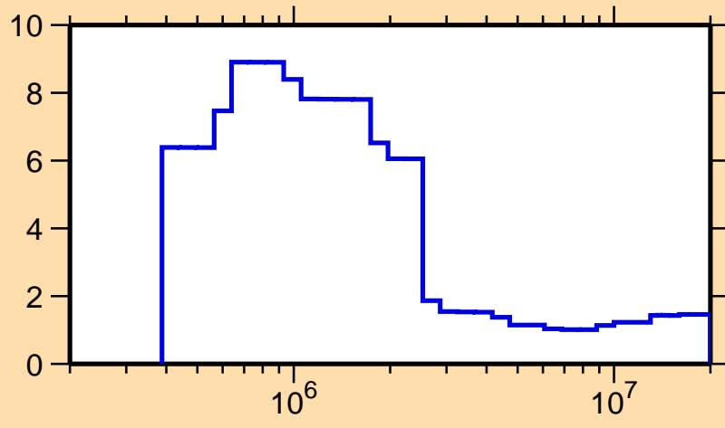
\Delta\sigma/\sigma vs. E for ^{130}\text{I}(n, nonel.)
