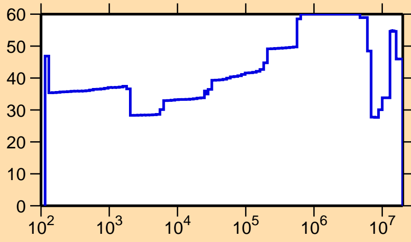
\Delta\sigma/\sigma vs. E for ^{130}\text{I}(n,\gamma)
