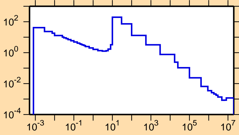
\sigma vs. E for ^{130}\text{I}(n,\gamma)
