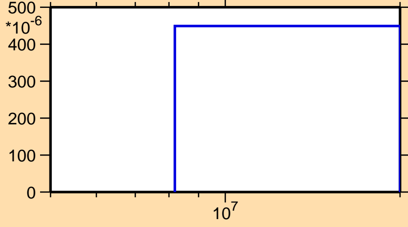
\sigma vs. E for ^{131}\text{I}(n,np)
