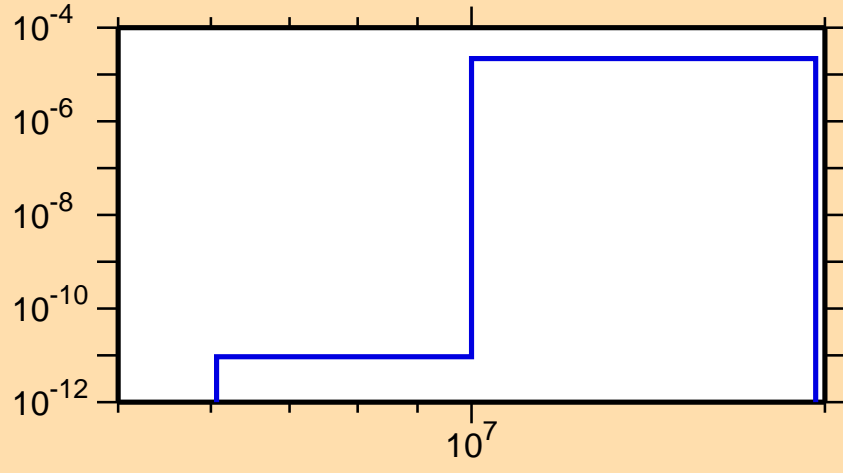
\sigma vs. E for ^{132}\text{I}(n,n\alpha)
