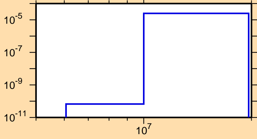
\sigma vs. E for ^{132}\text{I}(n,n\alpha)
