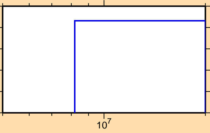
\sigma vs. E for ^{132}\text{I}(n,np)
