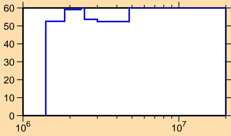
\Delta\sigma/\sigma vs. E for ^{132}\text{I}(n,n_1)
