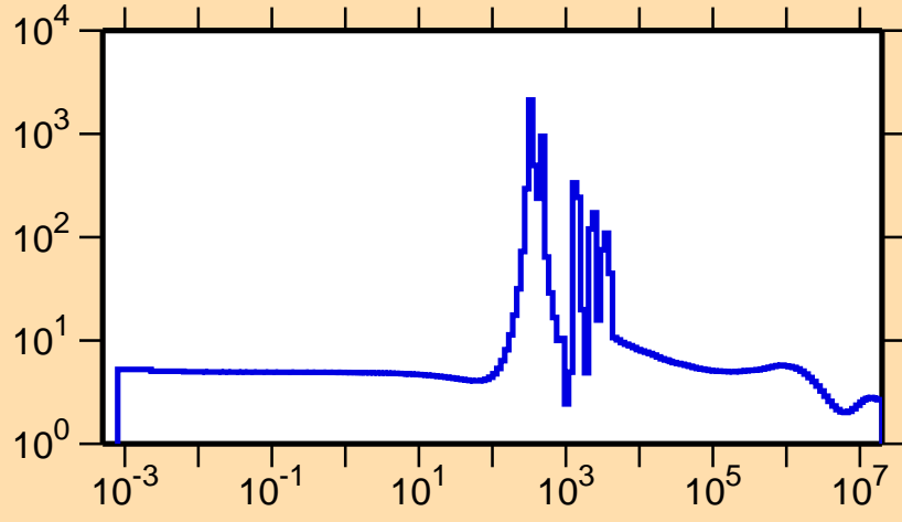
\sigma vs. E for ^{133}\text{I}(n,\text{el.})
