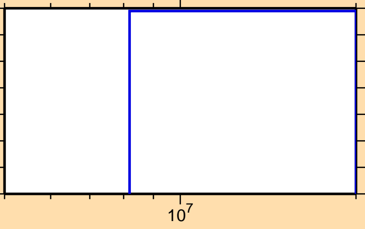
\sigma vs. E for ^{133}\text{I}(n,nt)
