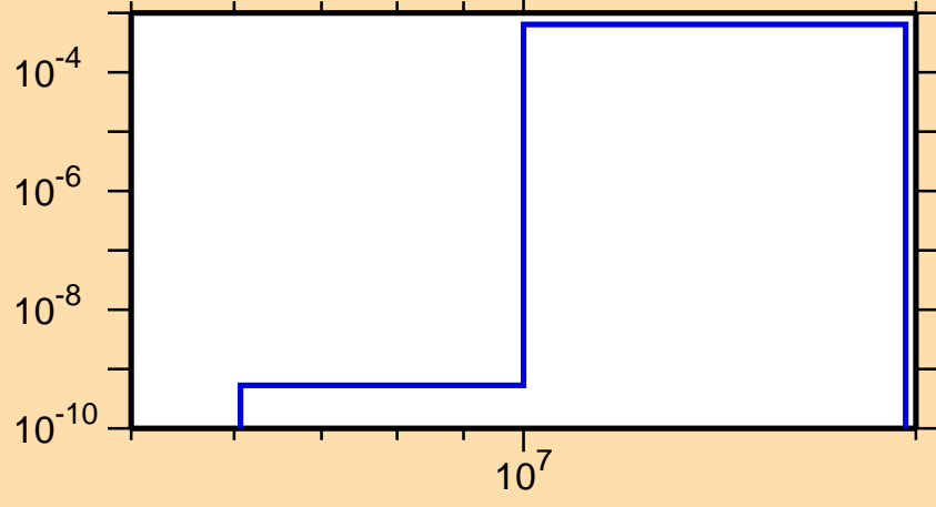
\sigma vs. E for ^{133}\text{I}(n,np)
