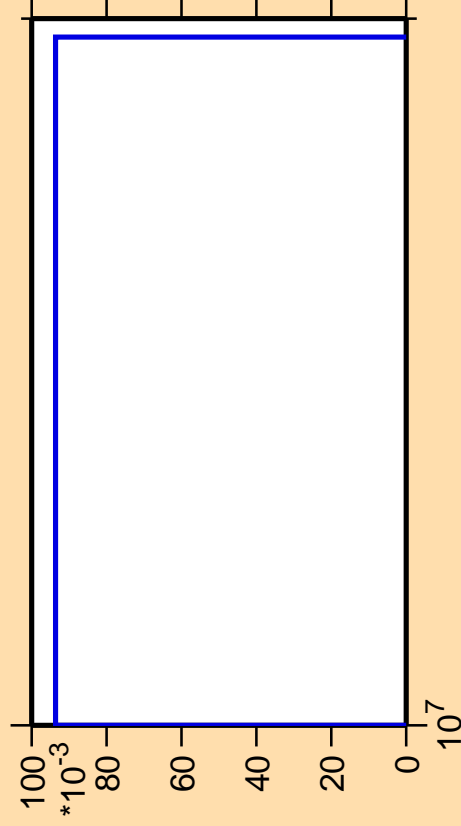
\Delta\sigma/\sigma vs. E for ^{133}\text{I}(n,p\alpha)
