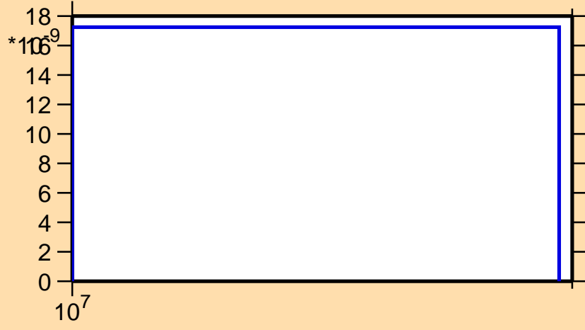
\sigma vs. E for ^{133}\text{I}(n,nt)
