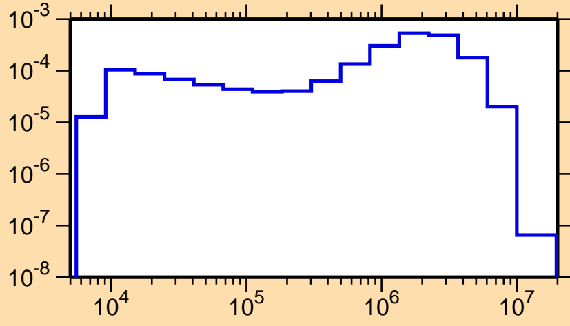
\sigma vs. E for ^{133}\text{I}(n,n_2)
