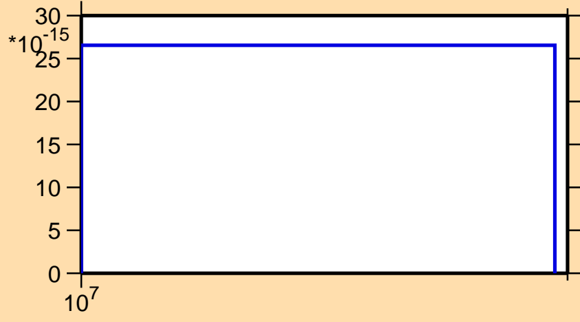
\sigma vs. E for ^{133}\text{I}(n,p\alpha)
