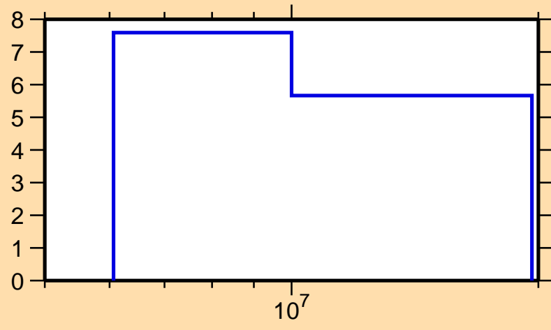
\Delta\sigma/\sigma vs. E for ^{133}\text{I}(n,\text{tot.})
