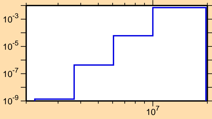
\sigma vs. E for ^{133}\text{I}(n,p)
