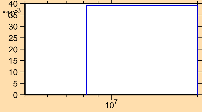
\sigma vs. E for ^{133}\text{I}(n,3n)
