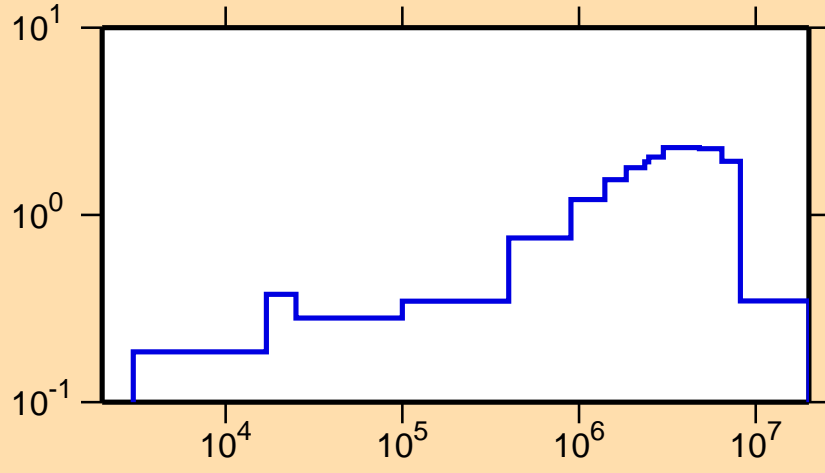
\sigma vs. E for ^{133}\text{I}(n,\text{inel.})
