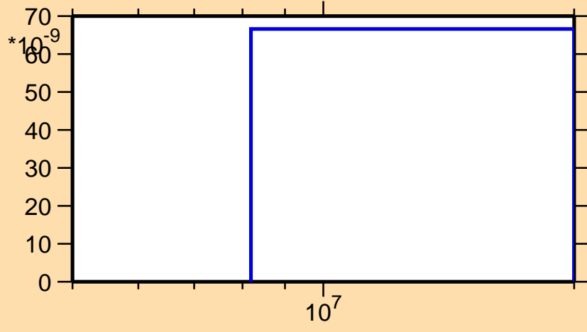
\sigma vs. E for ^{133}\text{I}(n,\text{nd})
