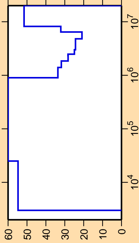
\Delta\sigma/\sigma vs. E for ^{133}\text{I}(n,\text{inel.})
