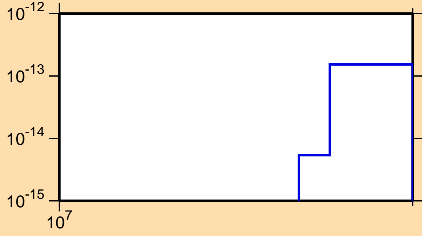
\sigma vs. E for ^{134}\text{I}(n,p\alpha)
