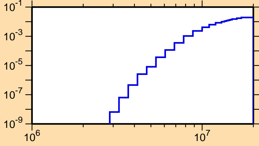
\sigma vs. E for ^{134}\text{I}(n,p)
