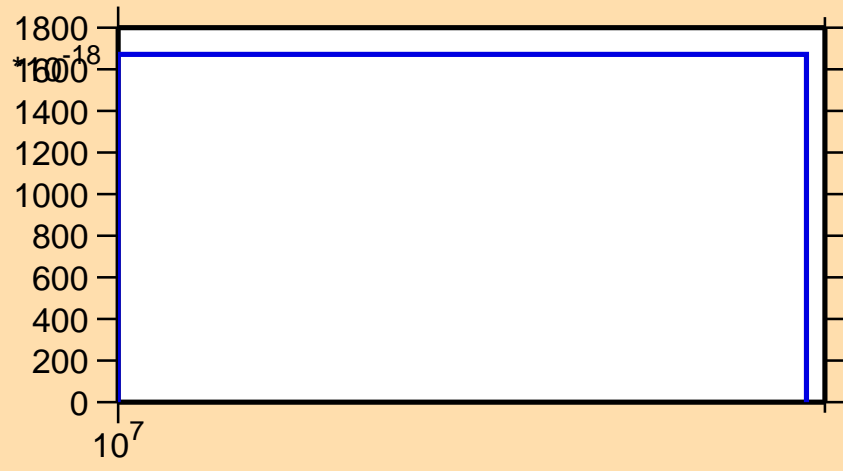
\sigma vs. E for ^{134}\text{I}(n,p\alpha)
