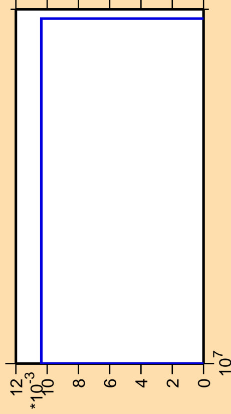
\Delta\sigma/\sigma vs. E for ^{134}\text{I}(n,p\alpha)
