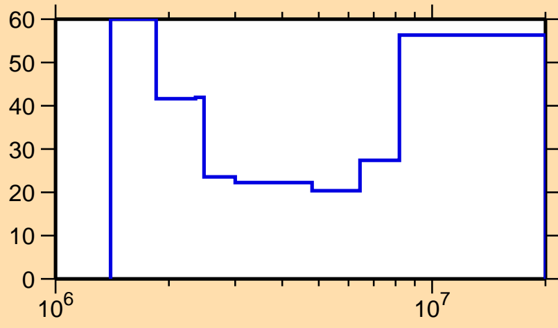
\Delta\sigma/\sigma vs. E for ^{134}\text{I}(n,ncont.)
