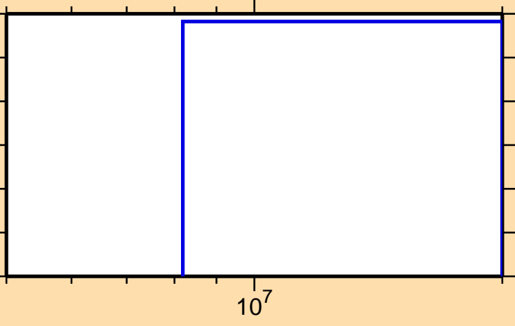
\sigma vs. E for ^{134}\text{I}(n,n\alpha)
