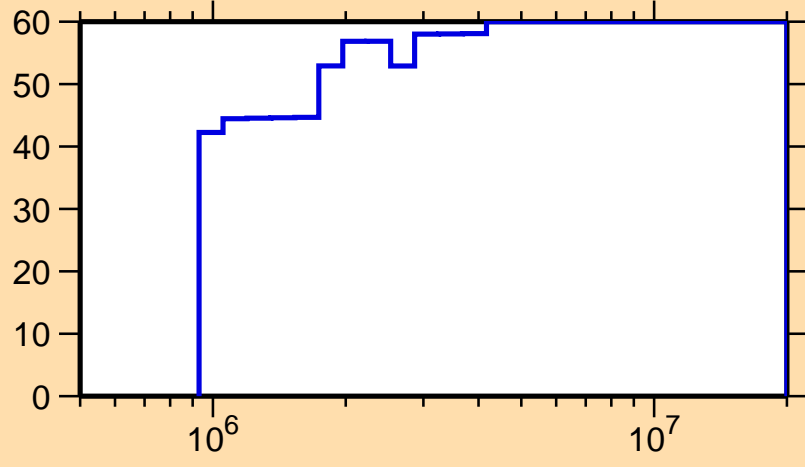
\Delta\sigma/\sigma vs. E for ^{134}\text{I}(n,\gamma)
