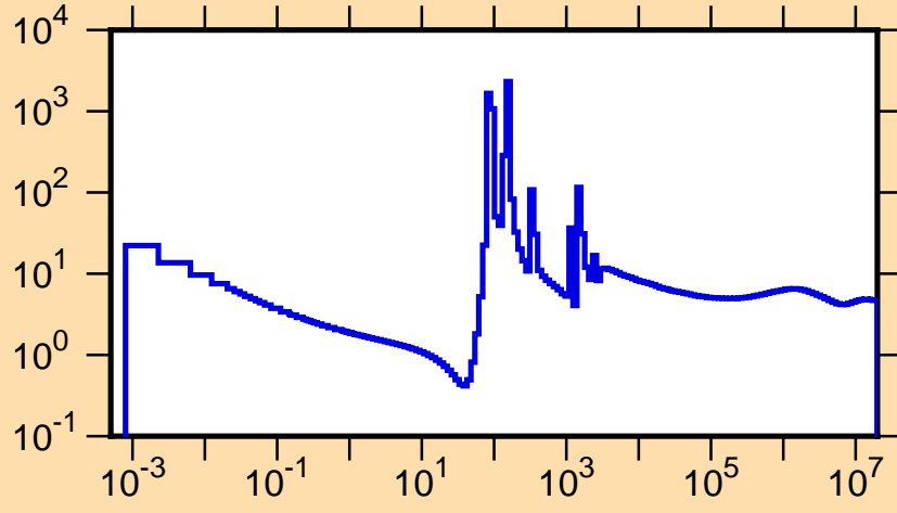
\sigma vs. E for ^{134}\text{I}(n,\text{tot.})
