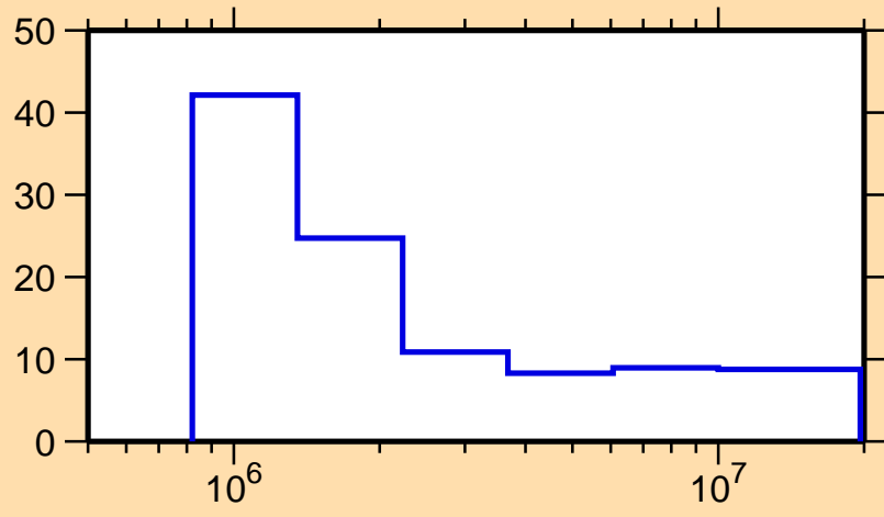
\Delta\sigma/\sigma vs. E for ^{134}\text{I}(n,n\text{nonel.})
