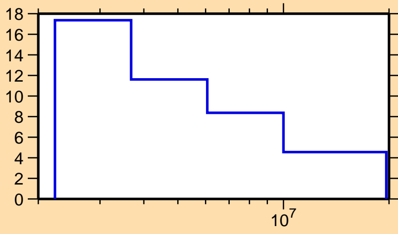
\Delta\sigma/\sigma vs. E for ^{134}\text{I}(n,el.)
