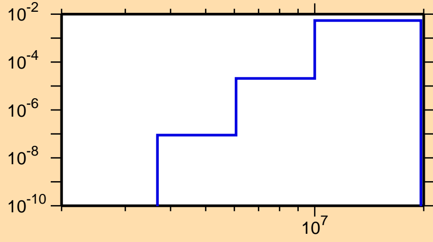
\sigma vs. E for ^{134}\text{I}(n,p)
