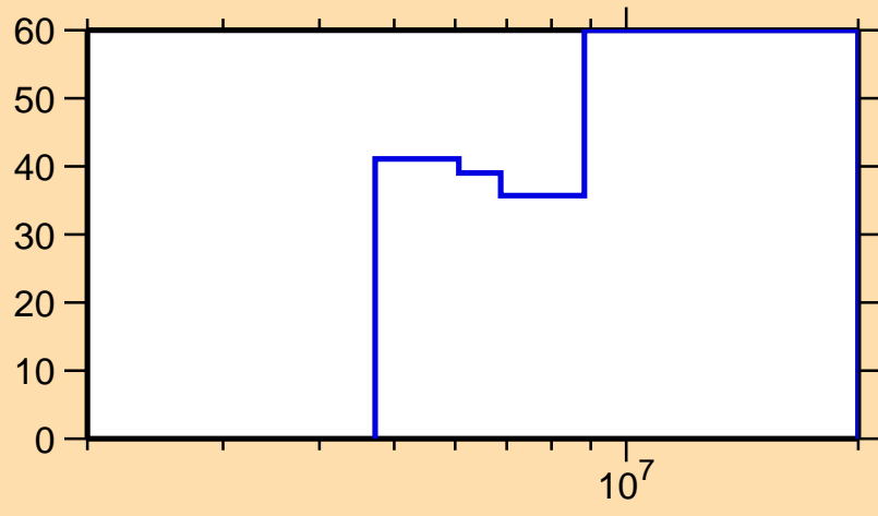
\Delta\sigma/\sigma vs. E for ^{135}\text{I}(n,n\text{cont.})
