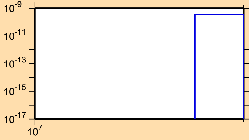
\sigma vs. E for ^{135}\text{I}(n,2np)
