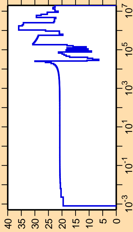
\Delta\sigma/\sigma vs. E for ^{135}\text{I}(n,\text{el.})
