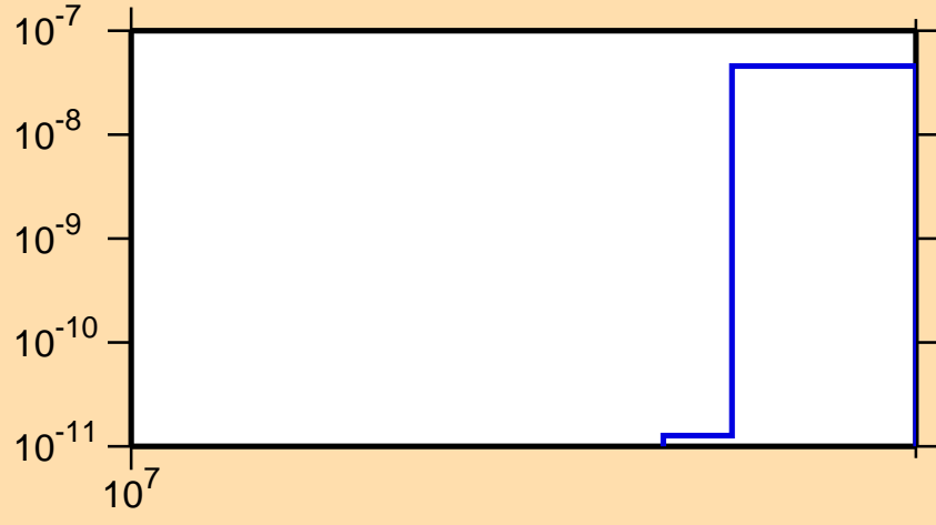
\sigma vs. E for ^{135}\text{I}(n,nt)
