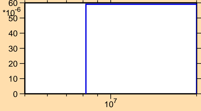
\sigma vs. E for ^{135}\text{I}(n,np)
