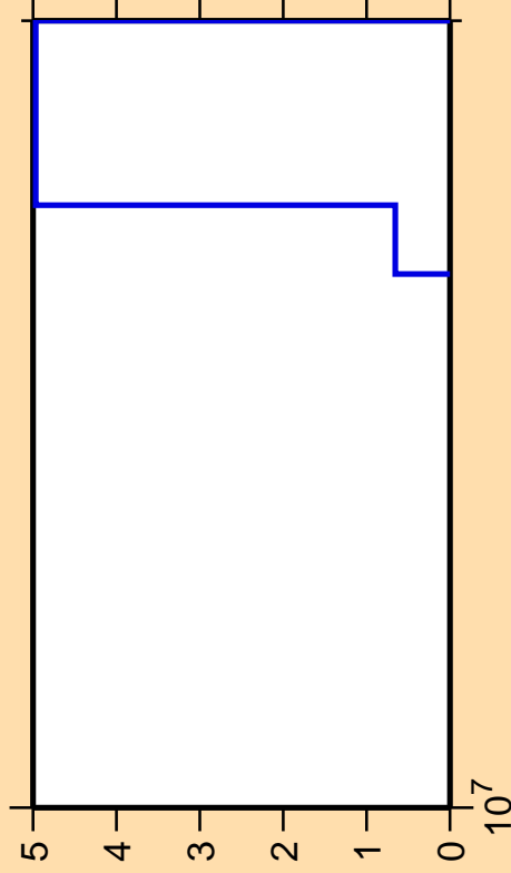
\Delta\sigma/\sigma vs. E for ^{136}\text{I}(n,p\alpha)
