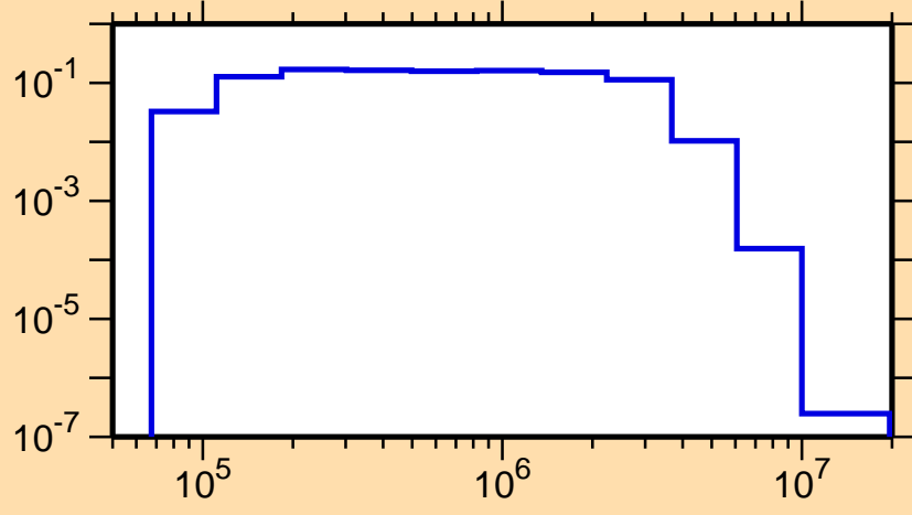
\sigma vs. E for ^{136}\text{I}(n,n_1)
