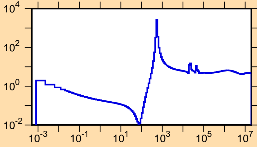
\sigma vs. E for ^{136}\text{I}(n,\text{tot.})
