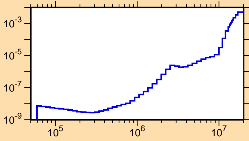
\sigma vs. E for ^{136}\text{I}(n,\alpha)
