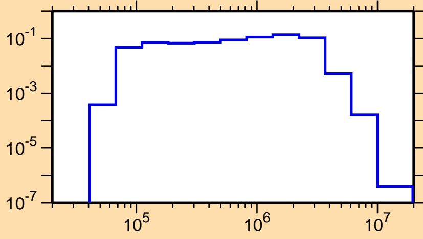
\sigma vs. E for ^{136}\text{I}(n,n_4)
