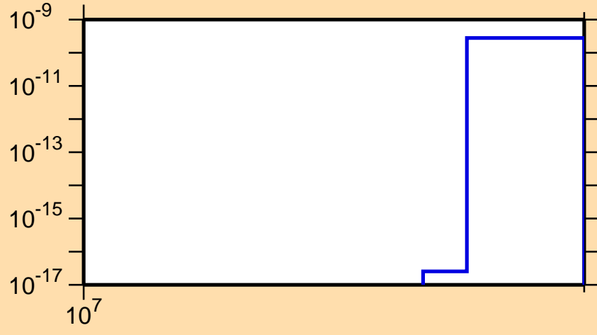
\sigma vs. E for ^{137}\text{I} (mt 11)
