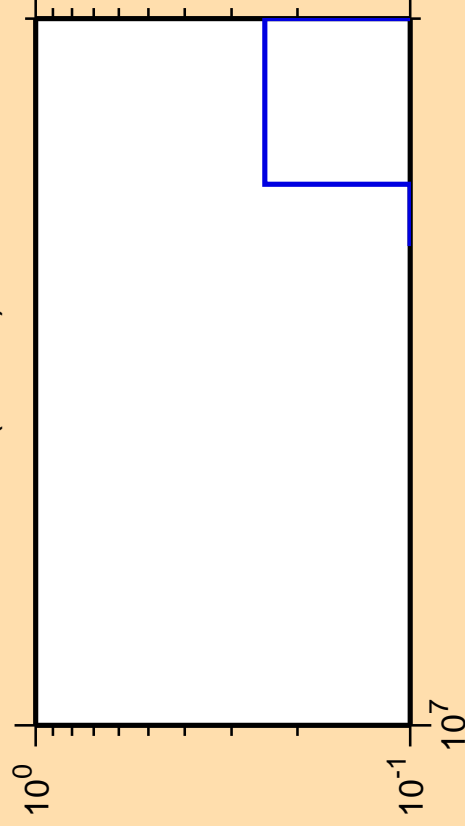
\Delta\sigma/\sigma vs. E for ^{137}\text{I}(n,3n\alpha)
