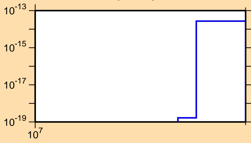
\sigma vs. E for ^{137}\text{I}(n,3n\alpha)
