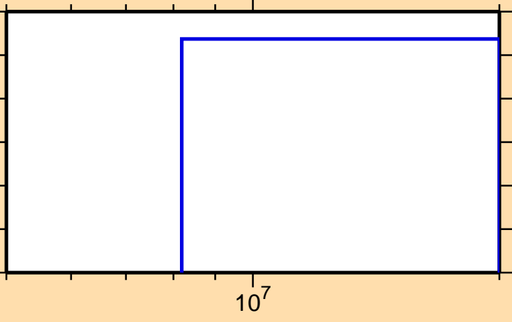
\sigma vs. E for ^{137}\text{I}(n,nt)
