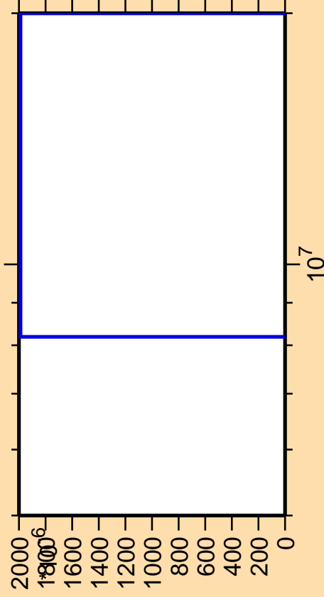
\Delta\sigma/\sigma vs. E for ^{137}\text{I}(n,3n\alpha)
