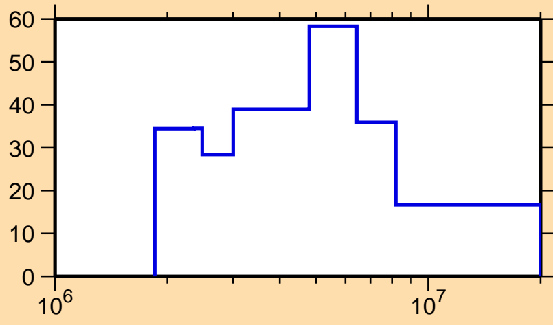
\Delta\sigma/\sigma vs. E for ^{137}\text{I}(n,el.)
