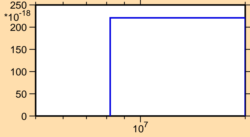
\sigma vs. E for ^{137}\text{I}(n,3n\alpha)
