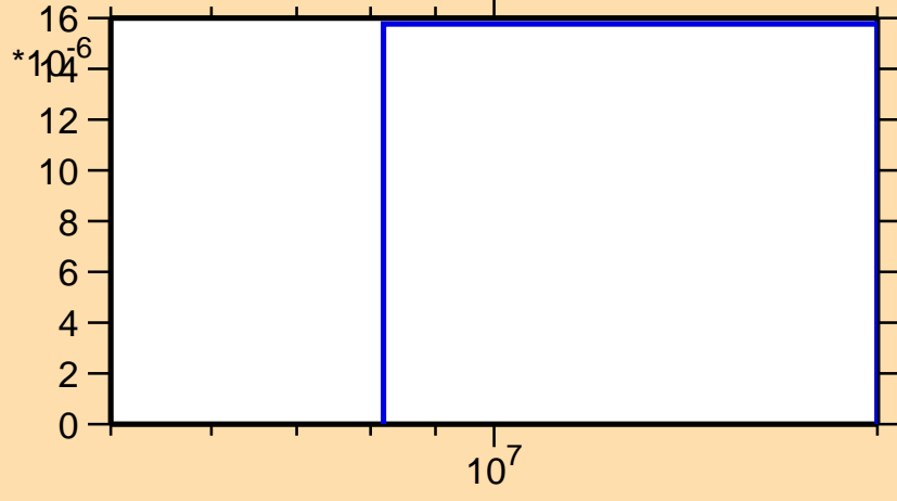
\sigma vs. E for ^{138}\text{I}(n,np)
