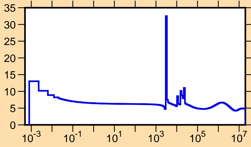
\sigma vs. E for ^{139}\text{I}(n,\text{tot.})
