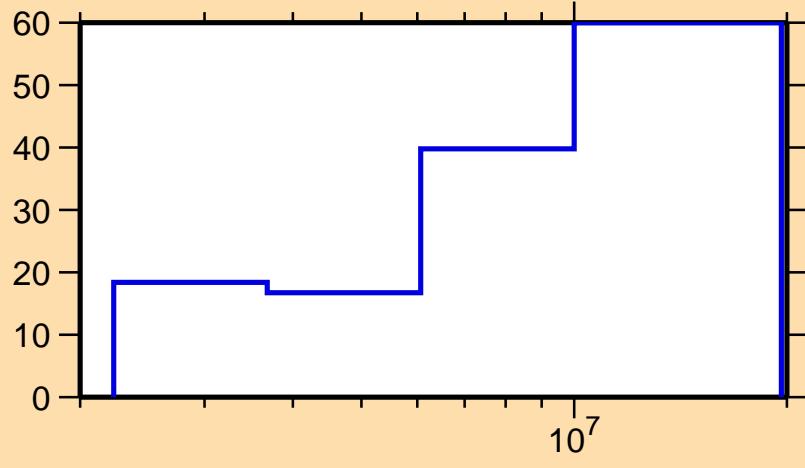
\Delta\sigma/\sigma vs. E for ^{139}\text{I}(n,n\text{cont.})
