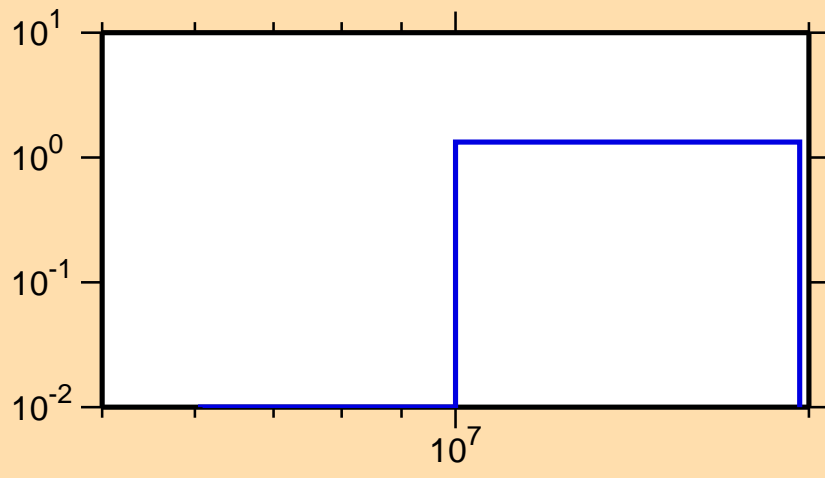
\sigma vs. E for ^{139}\text{I}(n,3n)
