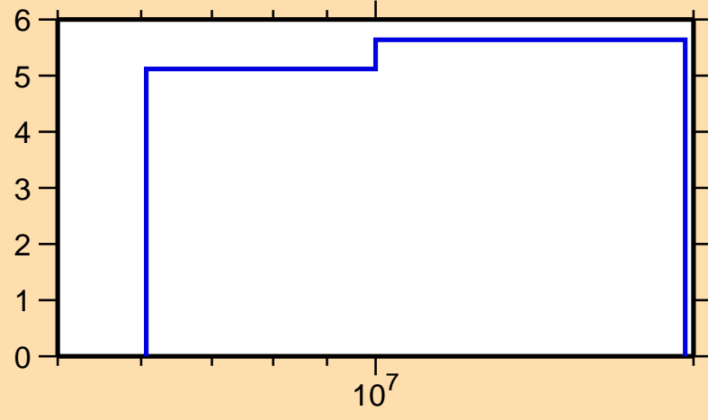
\Delta\sigma/\sigma vs. E for ^{139}\text{I}(n,\text{tot.})
