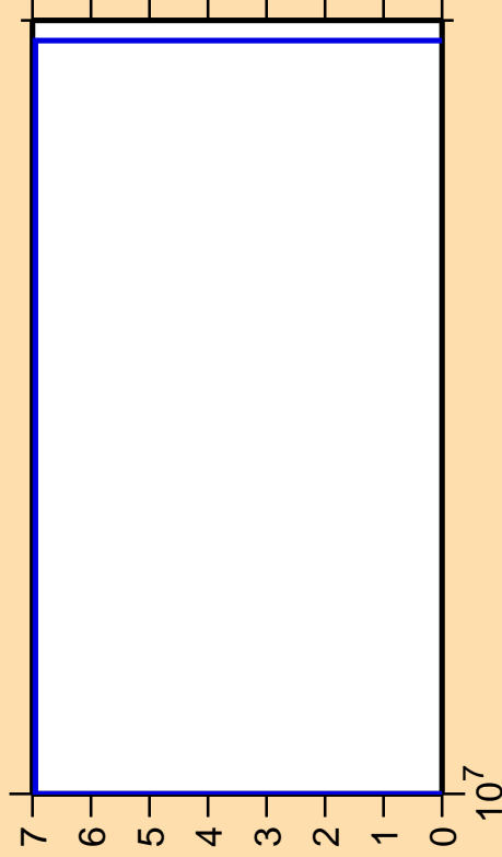
\Delta\sigma/\sigma vs. E for ^{139}\text{I} (mt 11)
