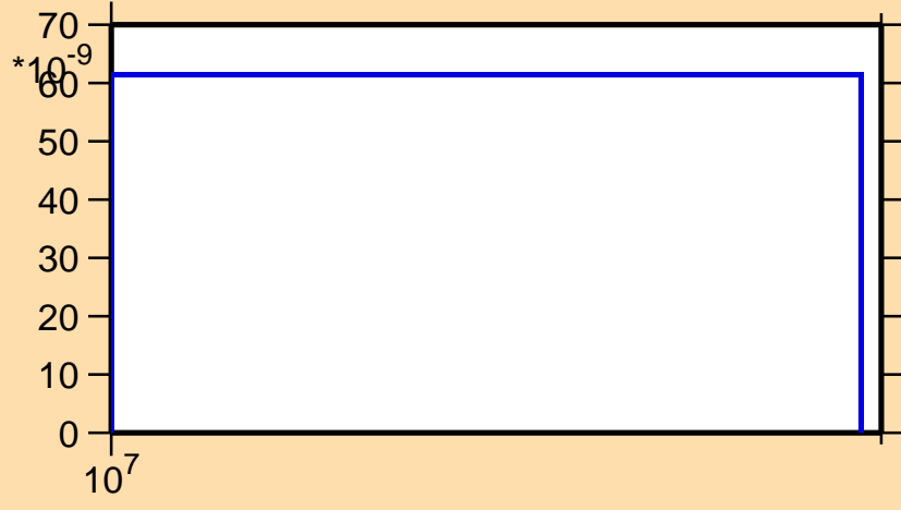
\sigma vs. E for ^{139}\text{I}(n,\text{nd})
