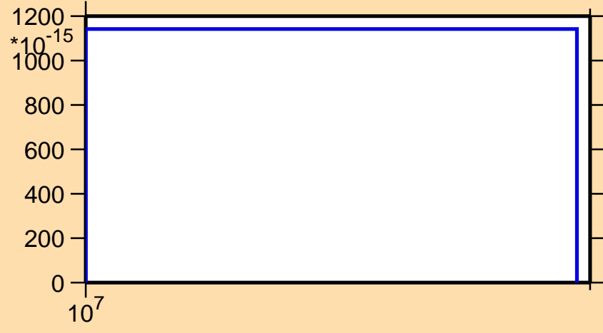
\sigma vs. E for ^{139}\text{I} (mt 11)
