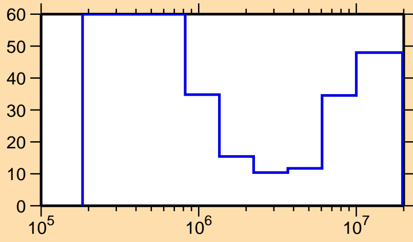
\Delta\sigma/\sigma vs. E for ^{139}\text{I}(n,\text{inel.})
