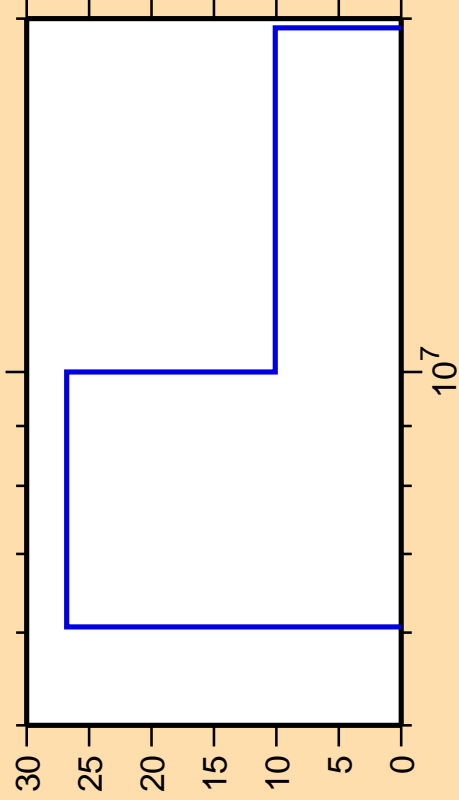
\Delta\sigma/\sigma vs. E for ^{139}\text{I}(n,3n)
