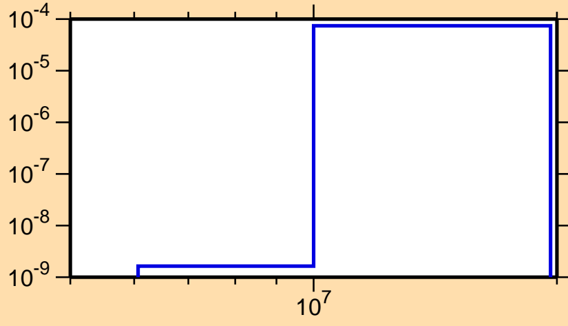
\sigma vs. E for ^{139}\text{I}(n,n\alpha)
