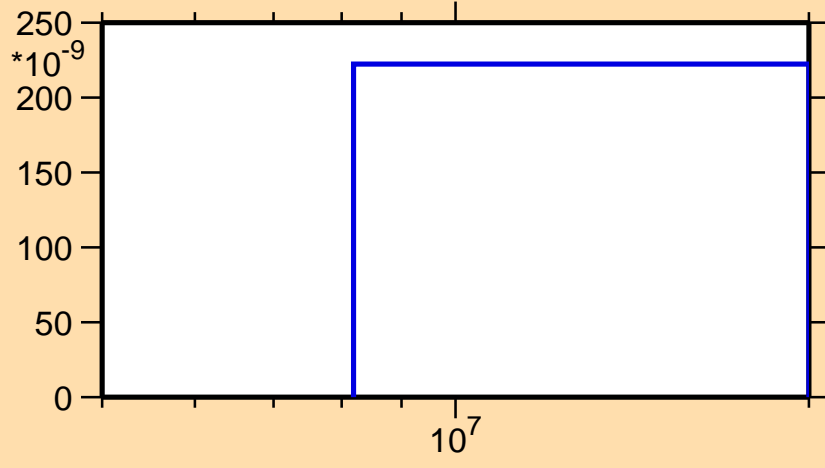
\sigma vs. E for ^{139}\text{I}(n,2n\alpha)
