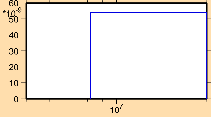
\sigma vs. E for ^{139}\text{I}(n,\text{nd})
