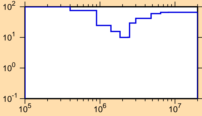
\Delta\sigma/\sigma vs. E for ^{139}\text{I}(n,n_1)
