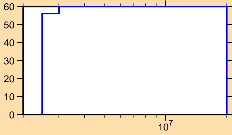
\Delta\sigma/\sigma vs. E for ^{139}\text{I}(n,\gamma)
