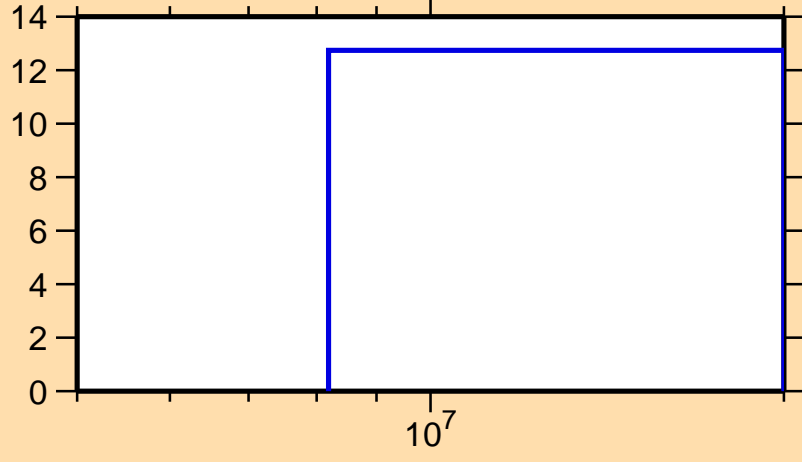
\Delta\sigma/\sigma vs. E for ^{139}\text{I}(n,el.)
