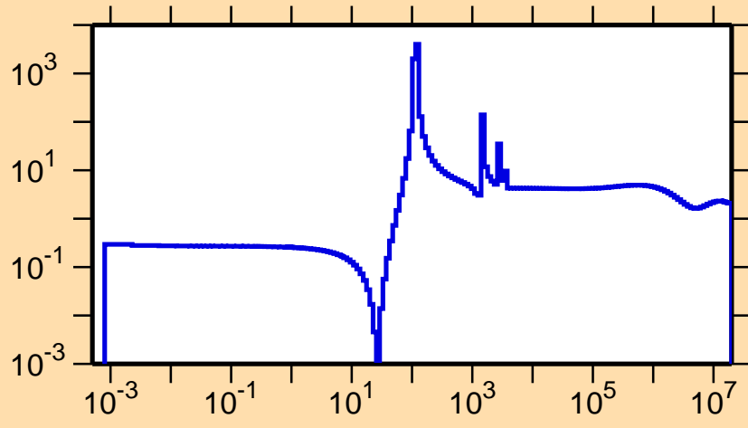
\sigma vs. E for ^{98}\text{In}(n,\text{el.})
