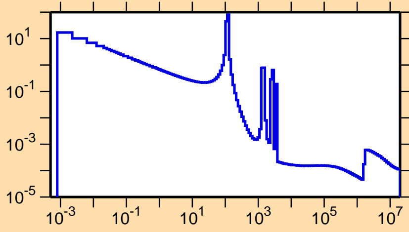
\sigma vs. E for ^{98}\text{In}(n,\gamma)
