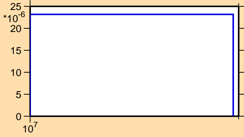
\sigma vs. E for ^{98}\text{In}(n,\text{pt})
