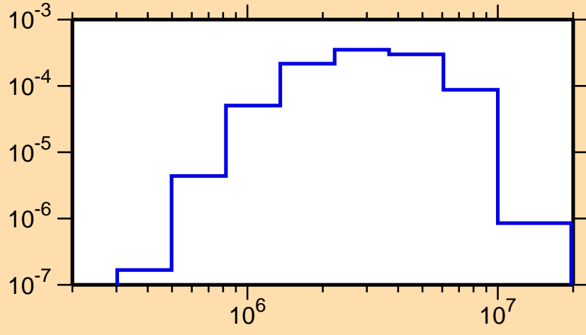
\sigma vs. E for ^{98}\text{In}(n,n_4)
