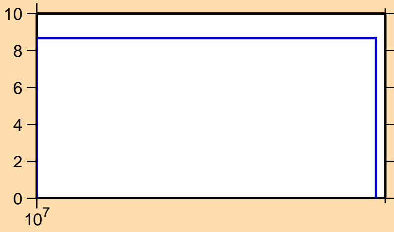
\Delta\sigma/\sigma vs. E for ^{98}\text{In}(n,\text{el.})
