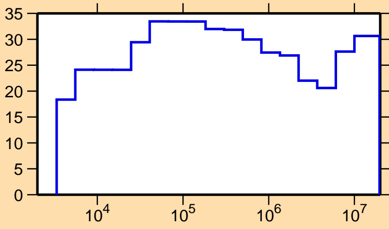
\Delta\sigma/\sigma vs. E for ^{98}\text{In}(n,p)
