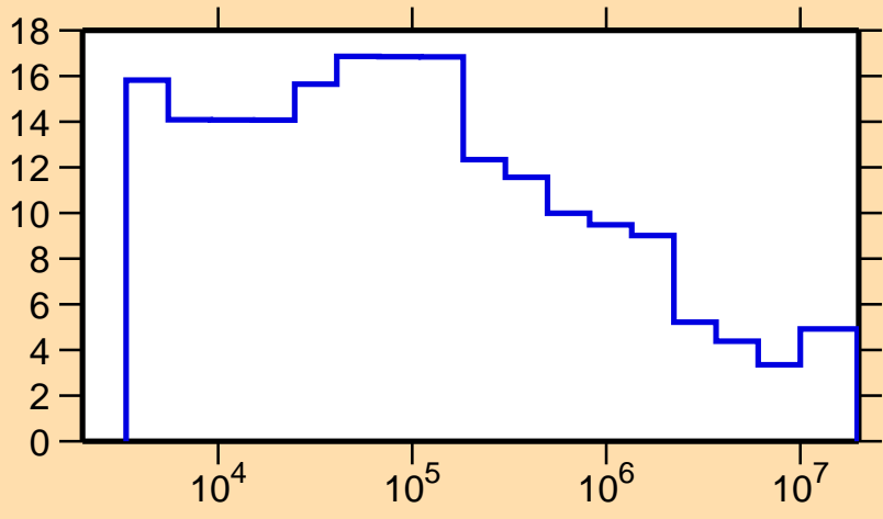
\Delta\sigma/\sigma vs. E for ^{98}\text{In}(n,\text{tot.})
