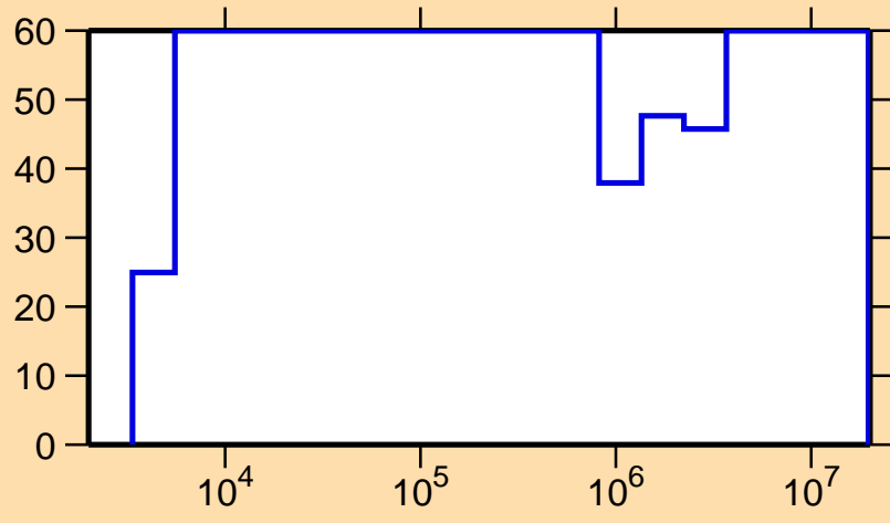
\Delta\sigma/\sigma vs. E for ^{98}\text{In}(n,\gamma)
