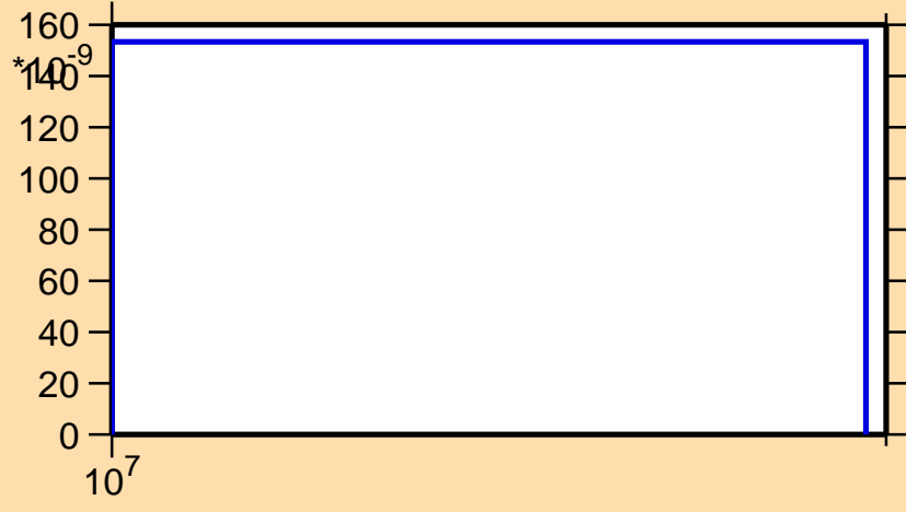
\sigma vs. E for ^{98}\text{In}(n,\text{nd})
