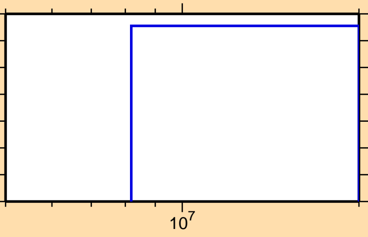
\sigma vs. E for ^{98}\text{In}(\text{mt117})
