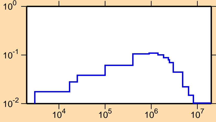
\sigma vs. E for ^{98}\text{In}(n,\text{inel.})
