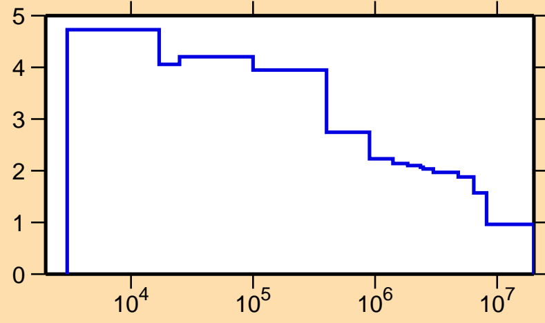
\sigma vs. E for ^{98}\text{In}(n,\text{nonel.})
