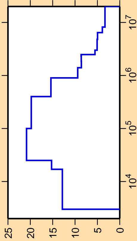
\Delta\sigma/\sigma vs. E for ^{98}\text{In}(n,\text{nonel.})
