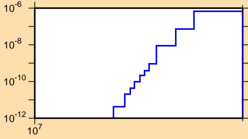
\sigma vs. E for ^{99}\text{In} (mt 45)
