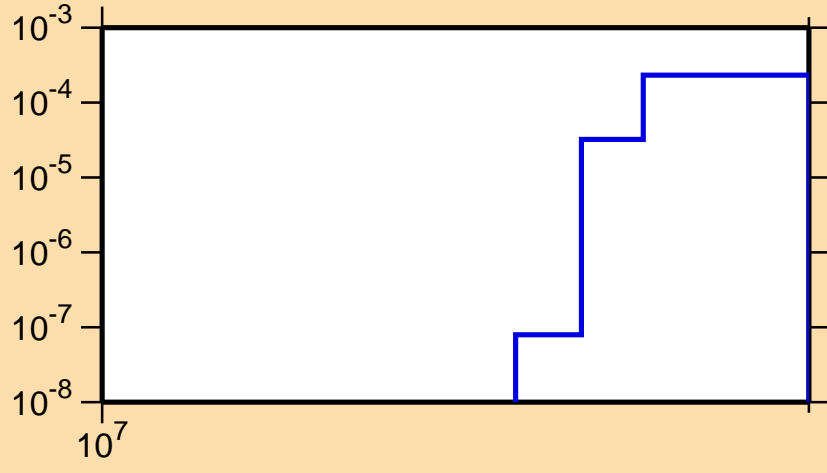
\sigma vs. E for ^{99}\text{In}(n,2n)
