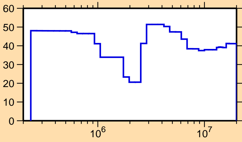
\Delta\sigma/\sigma vs. E for ^{99}\text{In}(n, el.)
