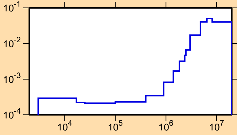
\sigma vs. E for ^{99}\text{In}(n,\alpha)
