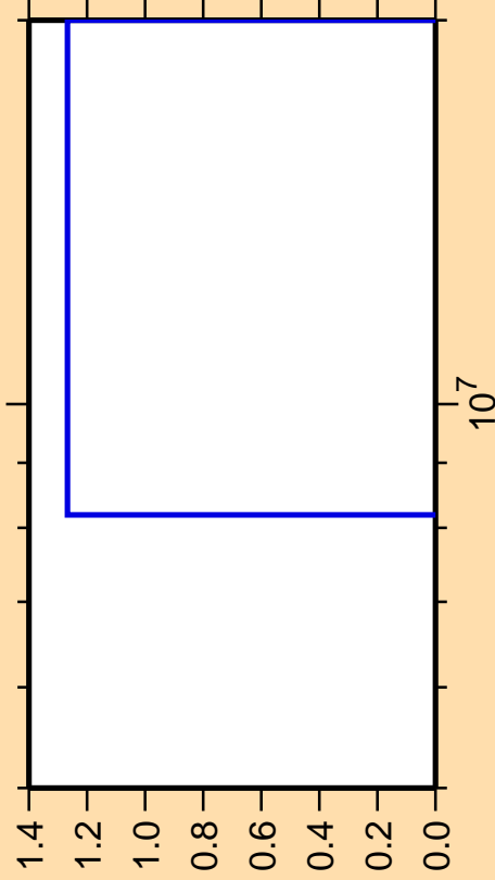
\Delta\sigma/\sigma vs. E for ^{99}\text{In}(\text{mt } 34)
