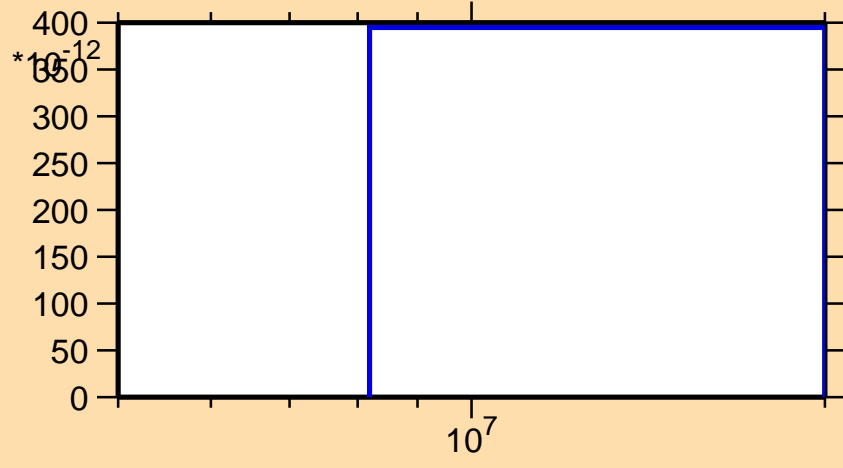
\sigma vs. E for ^{99}\text{In}(\text{mt117})
