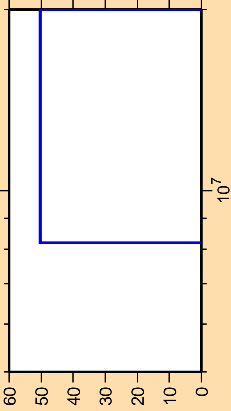
\Delta\sigma/\sigma vs. E for ^{99}\text{In}(n,2n)
