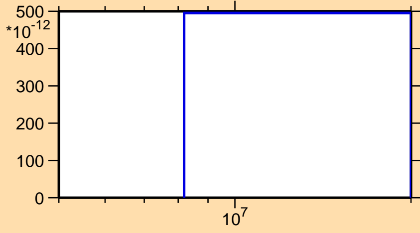
\sigma vs. E for ^{99}\text{In}(n,\text{nd})
