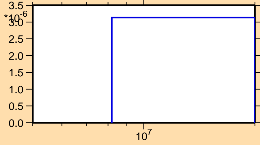
\sigma vs. E for ^{99}\text{In}(n,2n)
