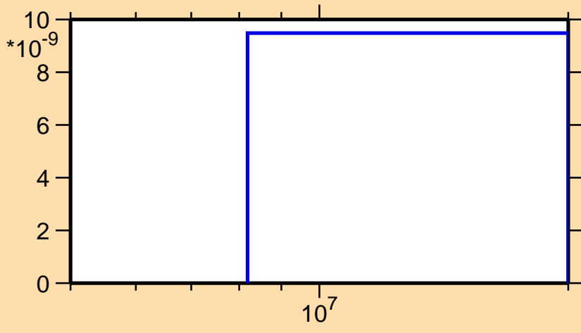
\sigma vs. E for ^{99}\text{In}(\text{mt } 45)
