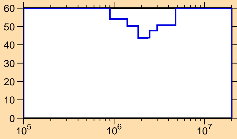
\Delta\sigma/\sigma vs. E for ^{99}\text{In}(n,n_1)
