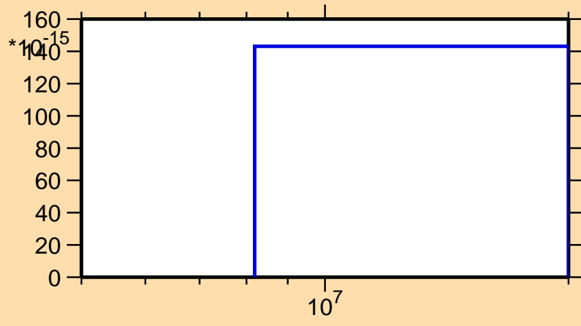
\sigma vs. E for ^{99}\text{In}(\text{mt } 34)
