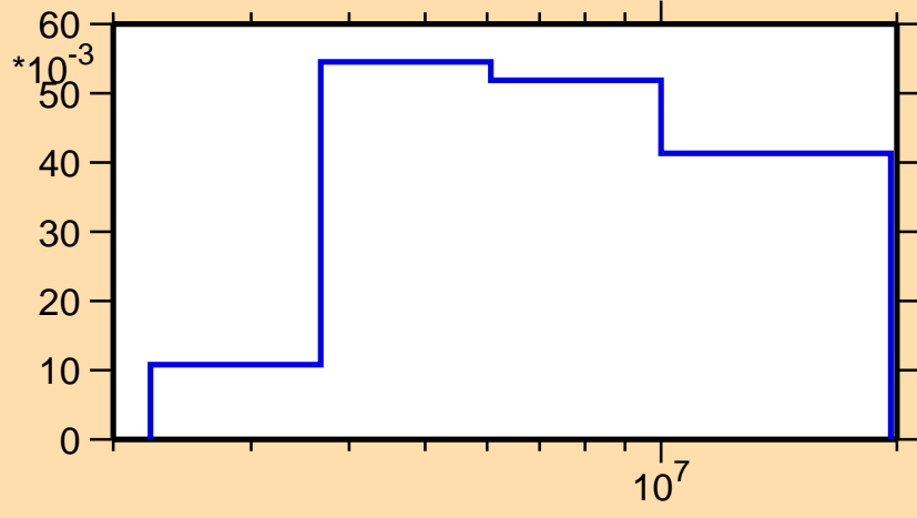
\sigma vs. E for ^{100}\text{In}(n,\text{inel.})
