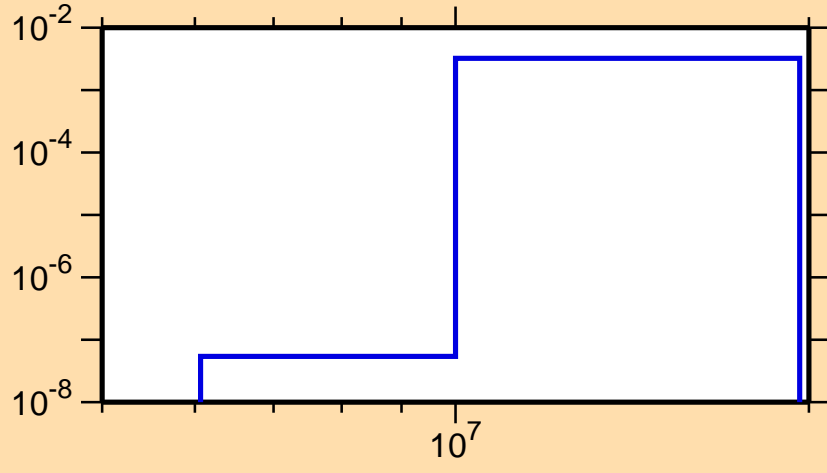
\sigma vs. E for ^{100}\text{In}(n,\text{pd})
