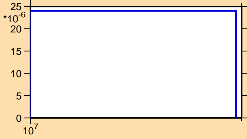
\sigma vs. E for ^{100}\text{In}(n,\text{pt})
