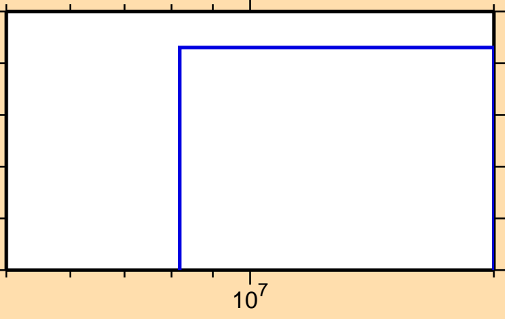
\sigma vs. E for ^{100}\text{In}(\text{mt117})
