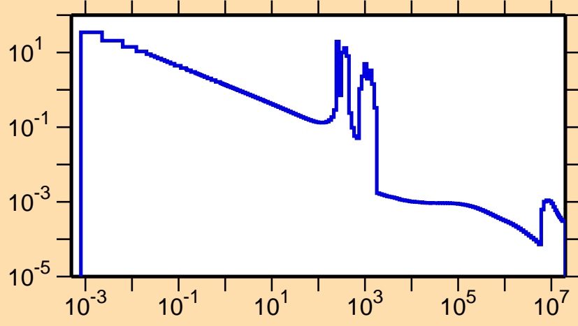
\sigma vs. E for ^{101}\text{In}(n,\gamma)
