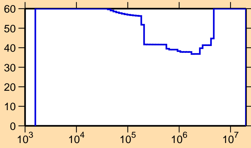
\Delta\sigma/\sigma vs. E for ^{101}\text{In}(n,p)
