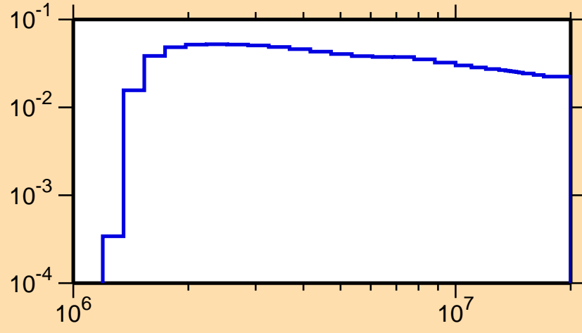
\sigma vs. E for ^{101}\text{In}(n,\text{inel.})
