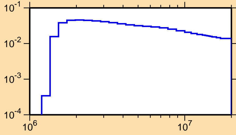
\sigma vs. E for ^{101}\text{In}(n,n_1)
