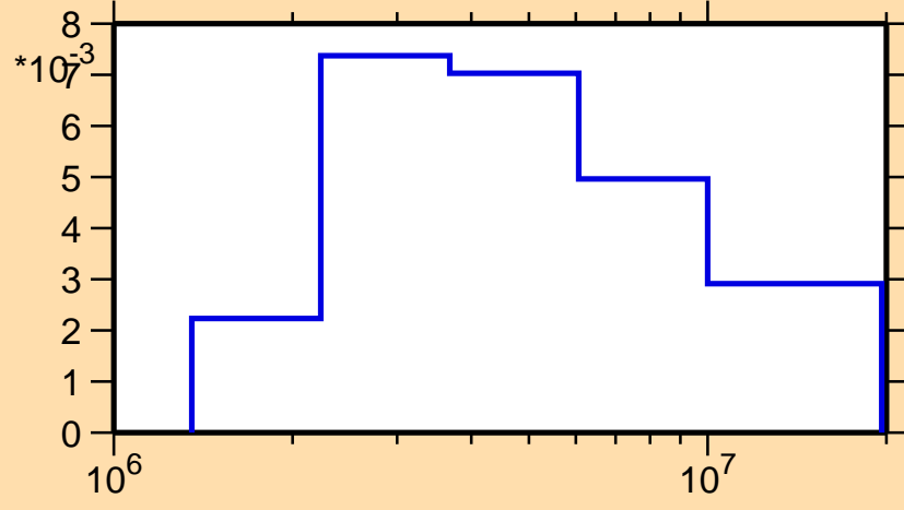
\sigma vs. E for ^{101}\text{In}(n,n_2)
