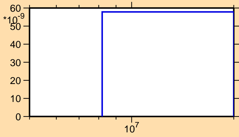
\sigma vs. E for ^{101}\text{In}(n,nd)
