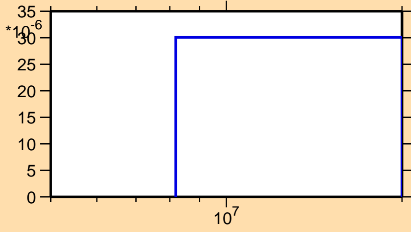
\sigma vs. E for ^{101}\text{In}(\text{mt } 45)
