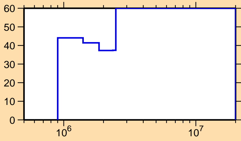
\Delta\sigma/\sigma vs. E for ^{101}\text{ln}(n, \text{el.})
