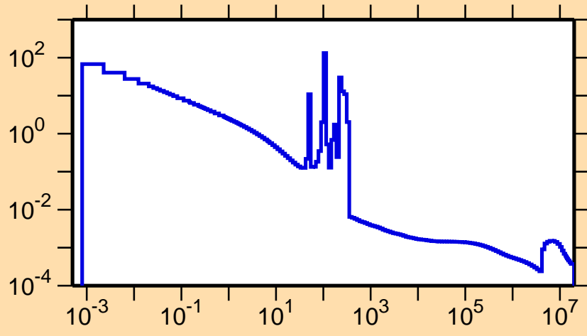
\sigma vs. E for ^{102}\text{In}(n,\gamma)
