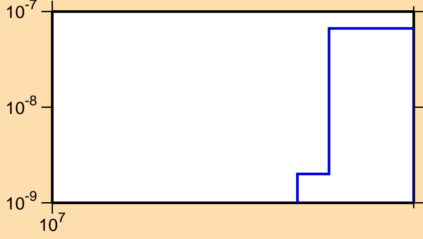
\sigma vs. E for ^{102}\text{In}(n,2n\alpha)
