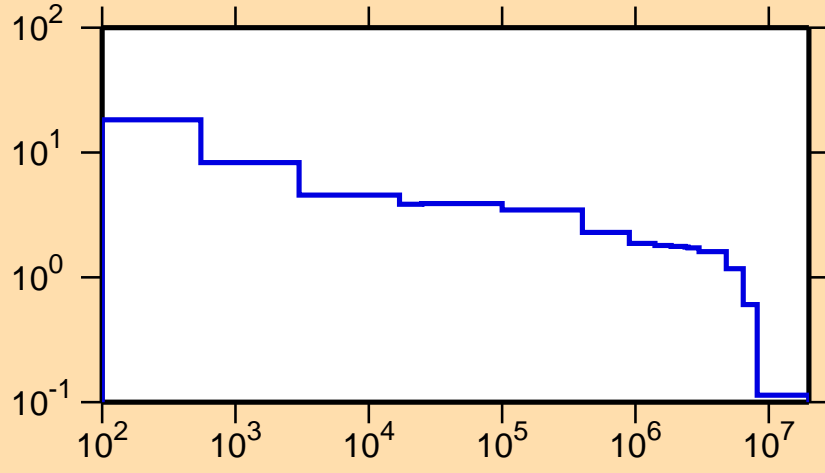
\sigma vs. E for ^{102}\text{In}(n,p)
