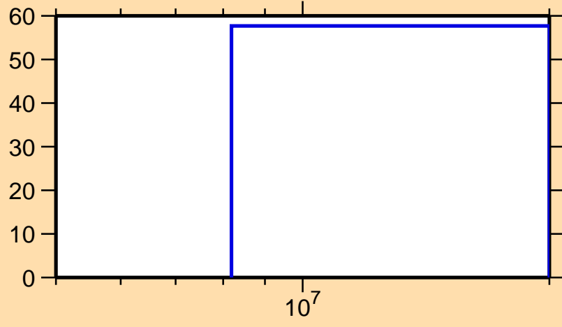
\Delta\sigma/\sigma vs. E for ^{102}\text{In}(n,\text{inel.})
