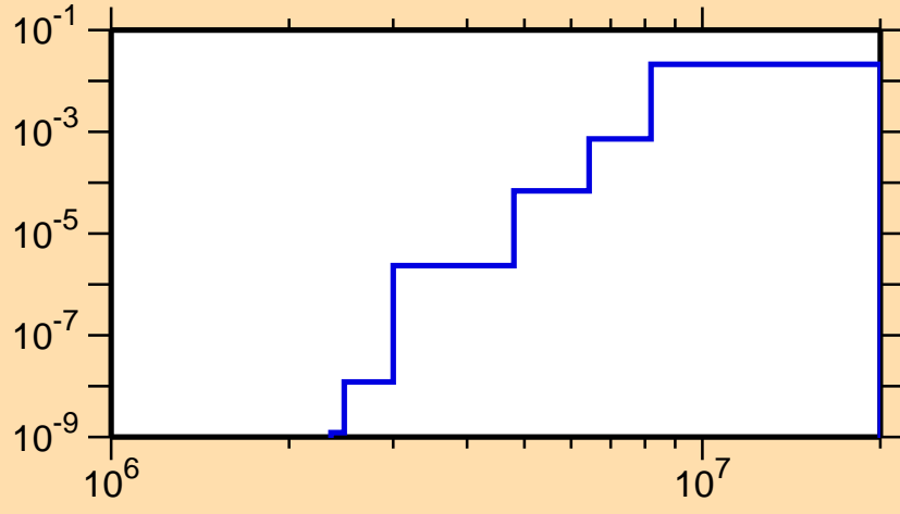
\sigma vs. E for ^{102}\text{In}(n,d)
