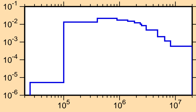
\sigma vs. E for ^{102}\text{In}(n,n_1)
