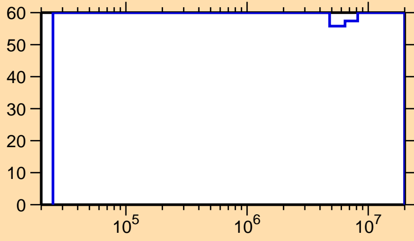
\Delta\sigma/\sigma vs. E for ^{102}\text{In}(n,n_1)
