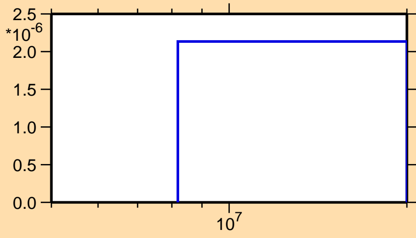
\sigma vs. E for ^{102}\text{In}(n,nd)
