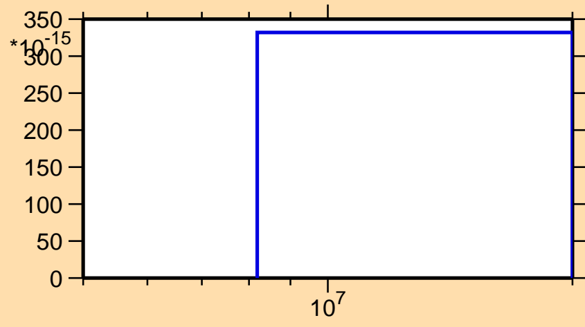
\sigma vs. E for ^{102}\text{In}(n,nt)
