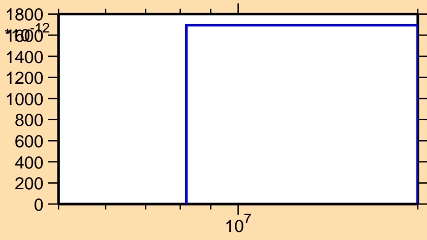
\sigma vs. E for ^{102}\text{In}(\text{mt } 34)
