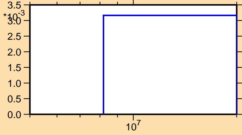
\sigma vs. E for ^{102}\text{In}(n,2n)
