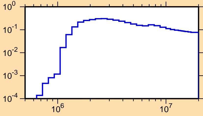
\sigma vs. E for ^{103}\text{In}(n,\text{inel.})
