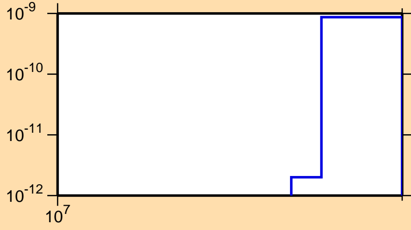
\sigma vs. E for ^{103}\text{In}(\text{mt } 34)
