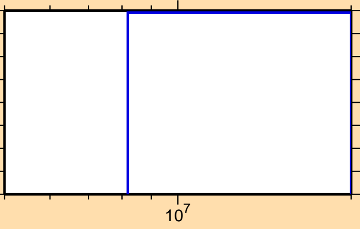
\sigma vs. E for ^{103}\text{In}(n,\text{pd})
